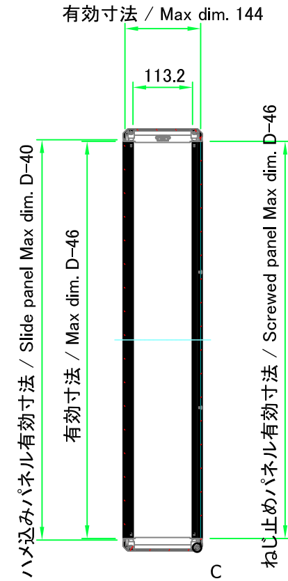
B-B (1:10)
